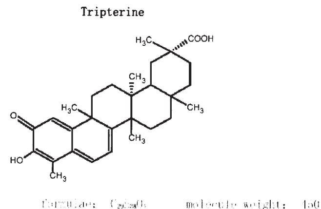
Fig. 1. Chemical structure and characteristics of tripterine. Origin from root of TWHF. Alternative name is celastrol. Determination of the structure: m.p.: 198~200°C. IR cm -1 : 3272, 2952, 1700, 1636, 1584. UV nm: 425. EI-MS m/z: 450 (M + , base peak), 241, 202. 1 H-NMR (CDCl 3 ) δ ppm: 0.57, 1.09, 1.25, 1.28, 1.43 (each 3H, s, CH 3 ), 2.21 (3H, s=C-CH 3 ), 6.32 (1H, d, J=7.3 Hz=CH), 6.49 (1H, d, J=1.2 Hz=CH), 7.06 (1H, dd, J=7.3/1.2 Hz=CH); 13 C-NMR (CDCl 3 ) δ ppm: 10.5q, 18.7q, 21.5q, 28.7t, 29.3qt, 29.5t, 30.7 s, 31.1t, 31.5q, 32.4q, 33.8t, 34.5t, 36.4t, 38.4q, 39.3 s, 39.9 s, 43.1 s, 44.3 d, 45.3 s, 118.3 d, 120.4 s, 120.6 d, 127.6 s, 135.4 d, 147.0 s, 165.0 s, 172.6 s, 178.3 s, 182.4 s. Purity determination. An external standard method by high-pressure liquid chromatography with Zorbax C 18 column as fixed phase and methanol-1% HAc (87:13) as mobile phase was adopted. The detection wavelength was 425 nm, the flow rate was 1.0 mL/min, and the purity was above 99.9%.
